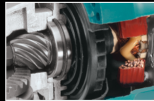
Makita's labyrinth construction seals and protects the motor from dust and debris
